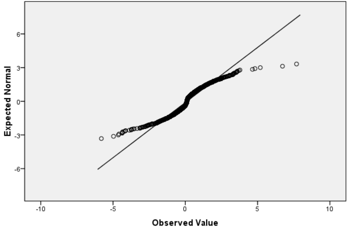
Normal Q-Q Plot of AGain
