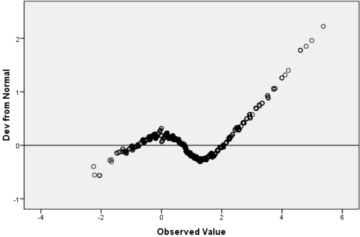
Detrended Normal Q-Q Plot of VGain
