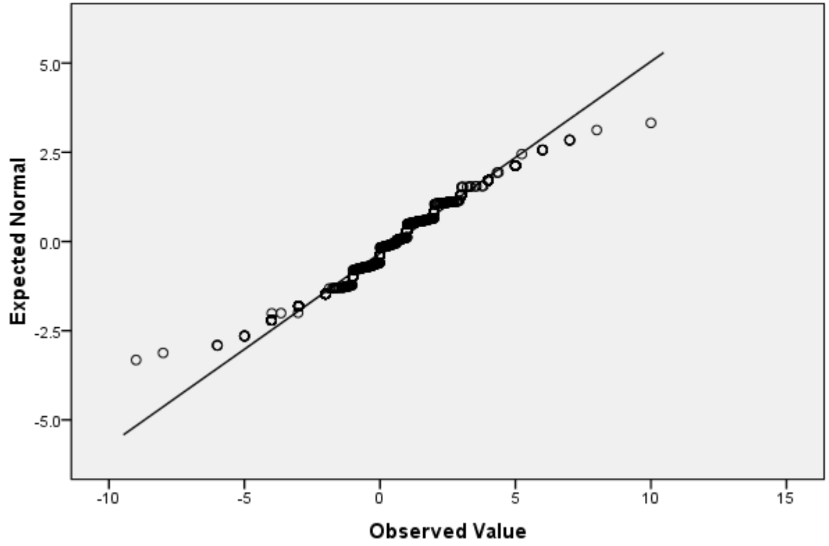
Normal Q-Q Plot of RGain
